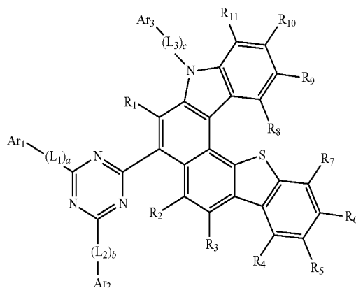
Formula 2d
