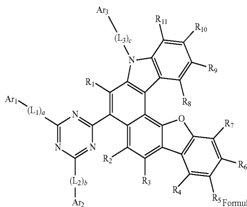
Formula 2c
