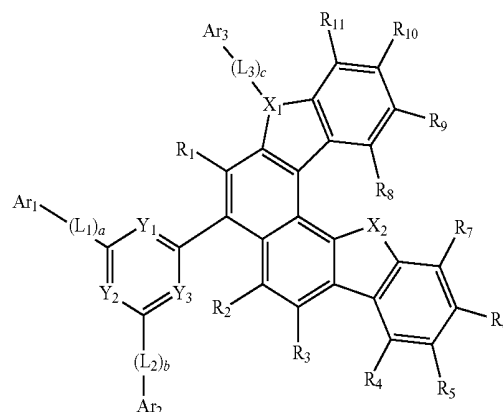
Formula 1
