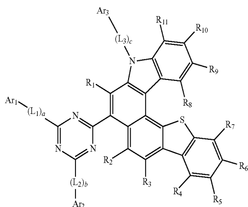
Formula 2b
