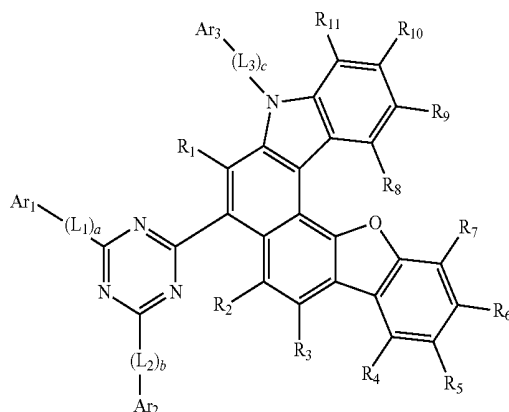
Formula 2c
