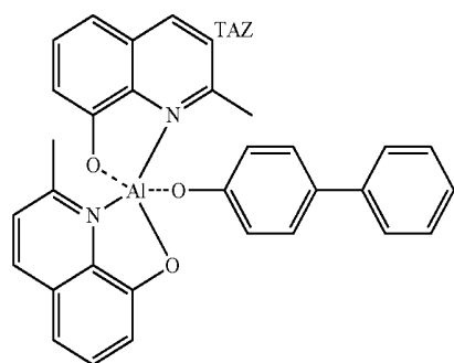
Compound 201
