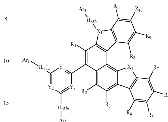
Formula 1
