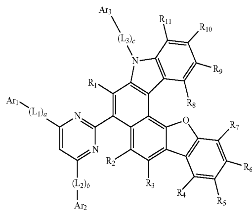
Formula 2f
