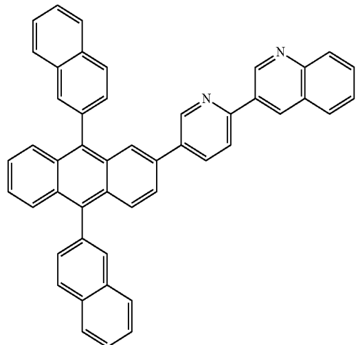
Compound 202
