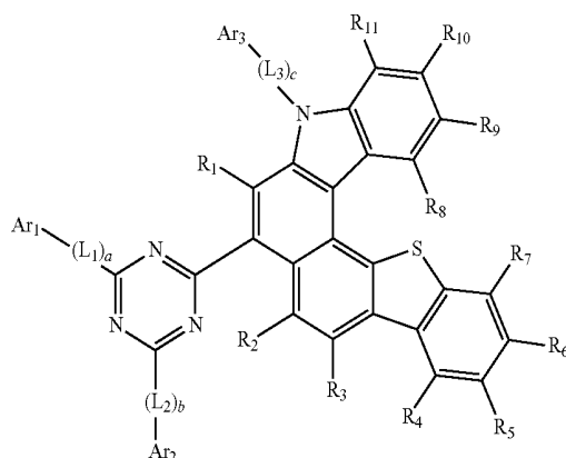
Formula 2b
