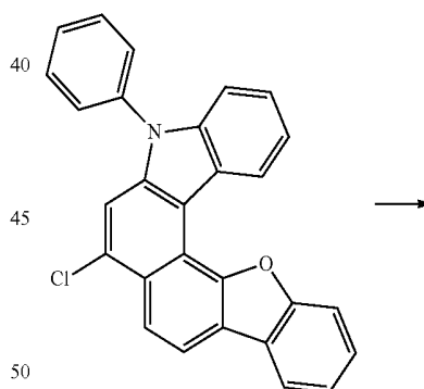
Reaction Scheme 3
