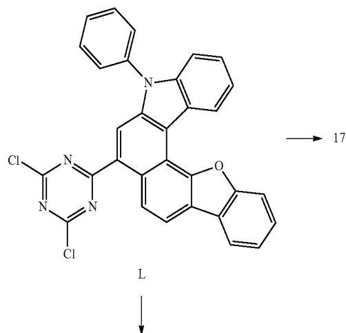
Reaction Scheme 4
