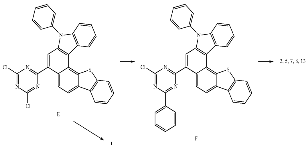
Reaction Scheme 2
