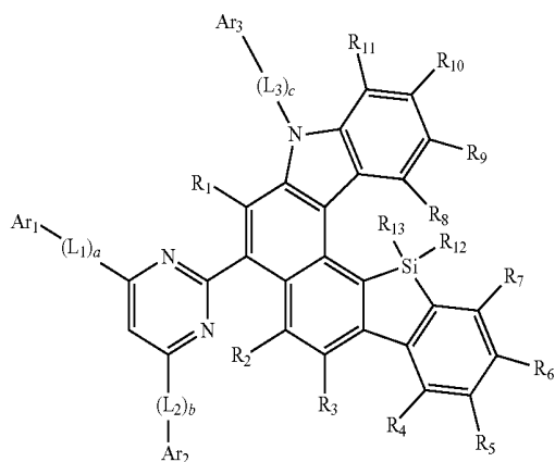
Formula 2f
