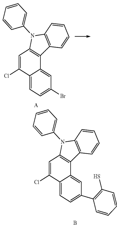
Reaction Scheme 1
